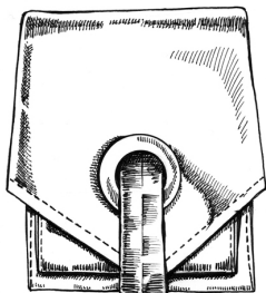
Closed Front
