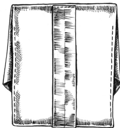
Closed Back
