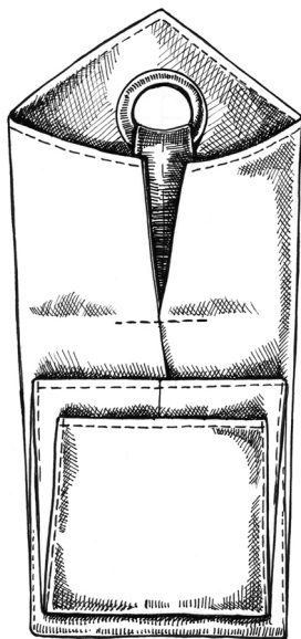
Open
